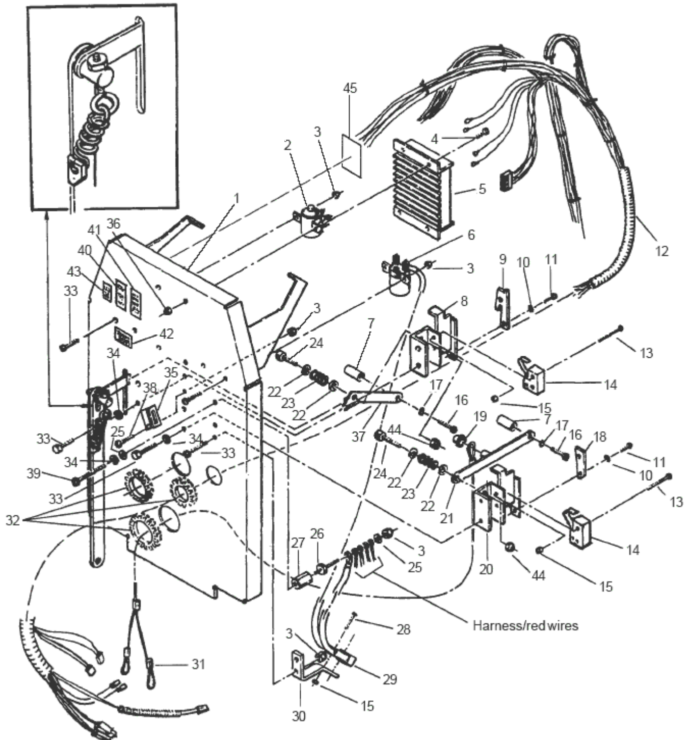
CLARKTECHNOLOGY Encore S20/L20 Rear Panel Assembly Drawing 11/01 (for machines with a 41150B traverse controller)
